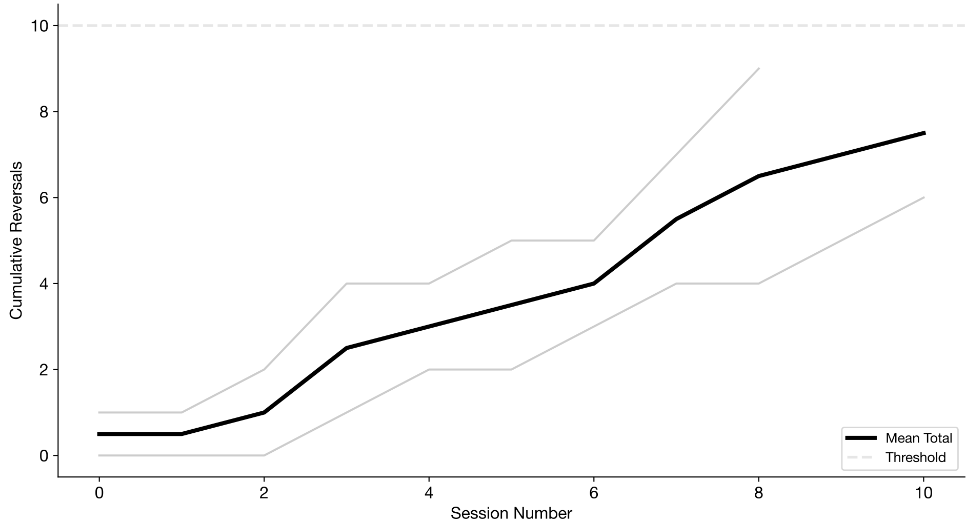
Cumulative Total Reversals Over Time (n=2 subjects; sessions per subject=9–11)
